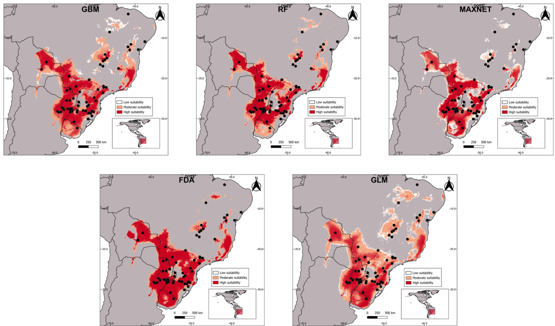
Fig. S1. Individual model predictions for each algorithm used in the bioclimatic model (GBM, RF, MAXNET, FDA, and GLM), showing habitat suitability for Paspalum guenoarum .
